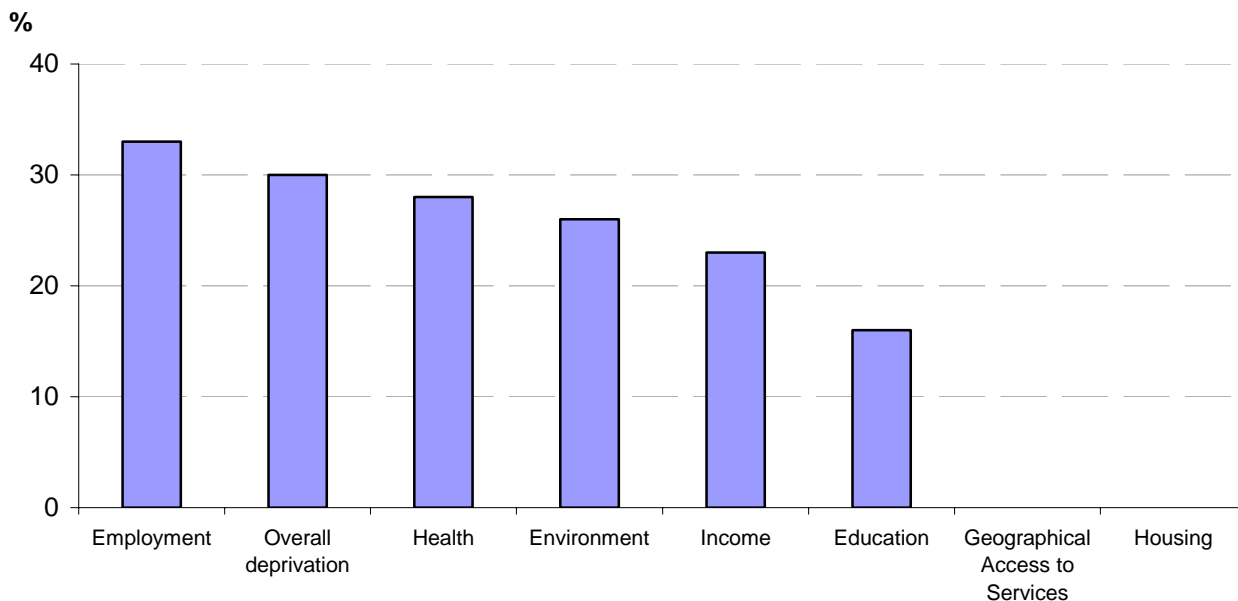
Figure 1: The % of LSOAs in Aberavon that are in the 10% most deprived LSOAs in Wales, for overall deprivation and by domain, 2005
